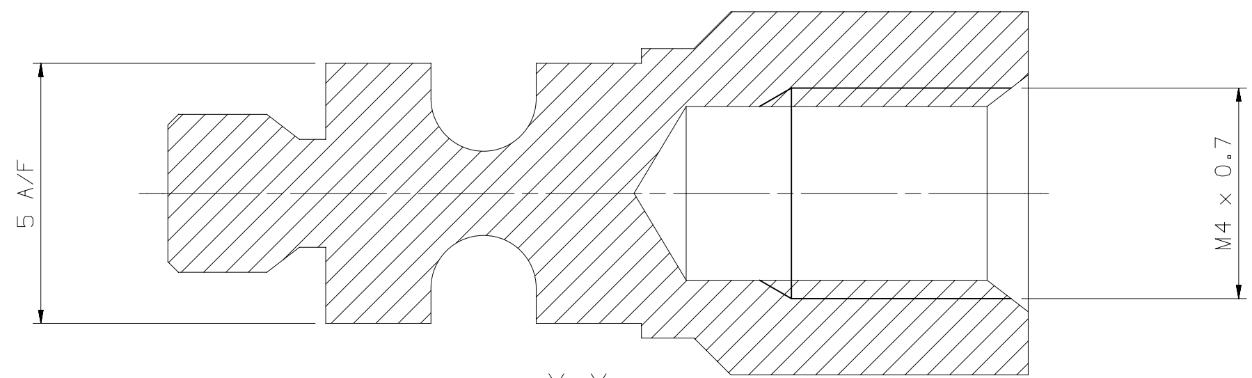
SECTION X-X
